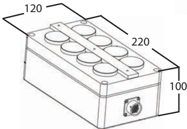
Tray Diminsions
